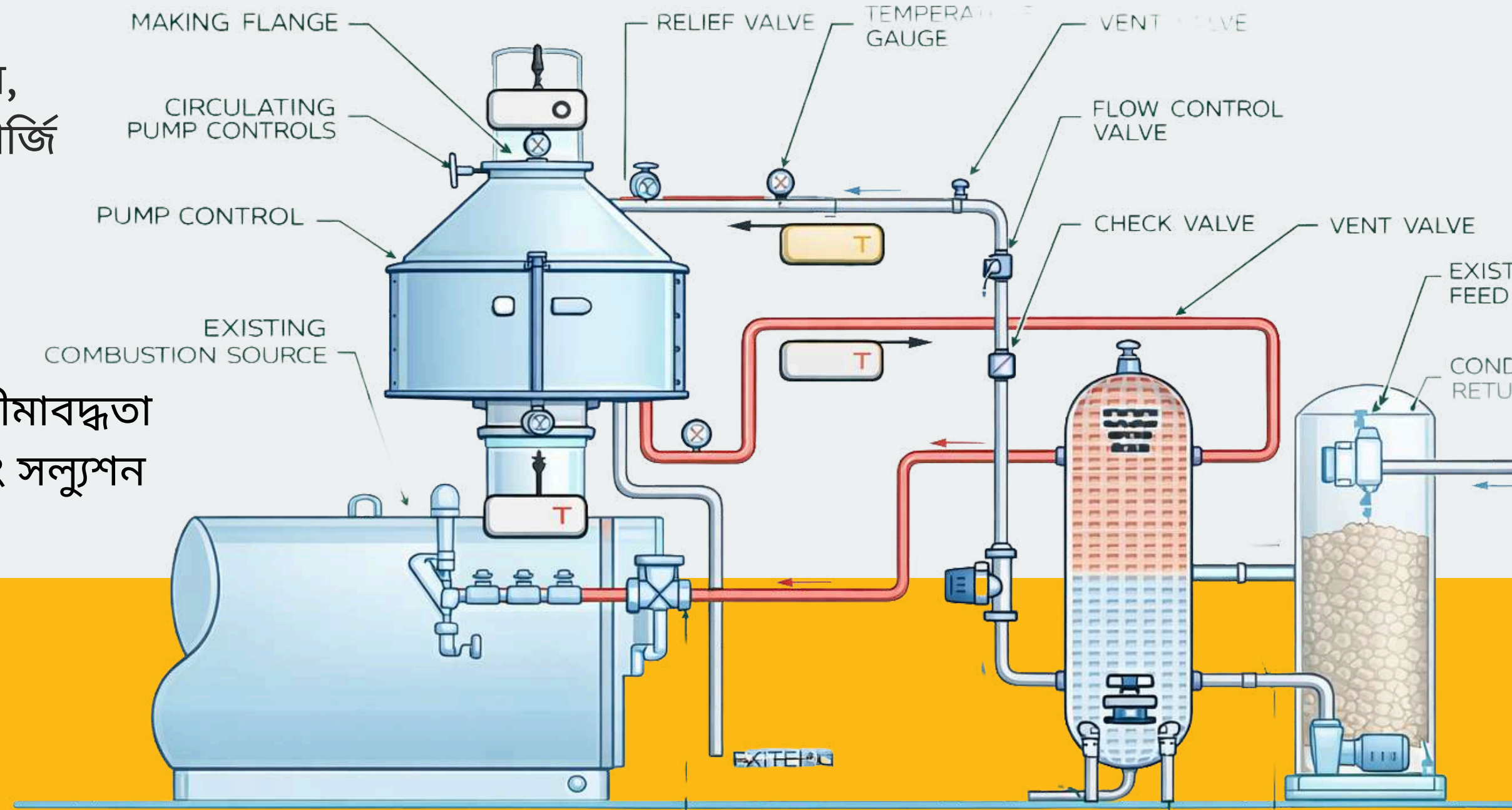
Fig: Boiler Feed System Schematic Overview
